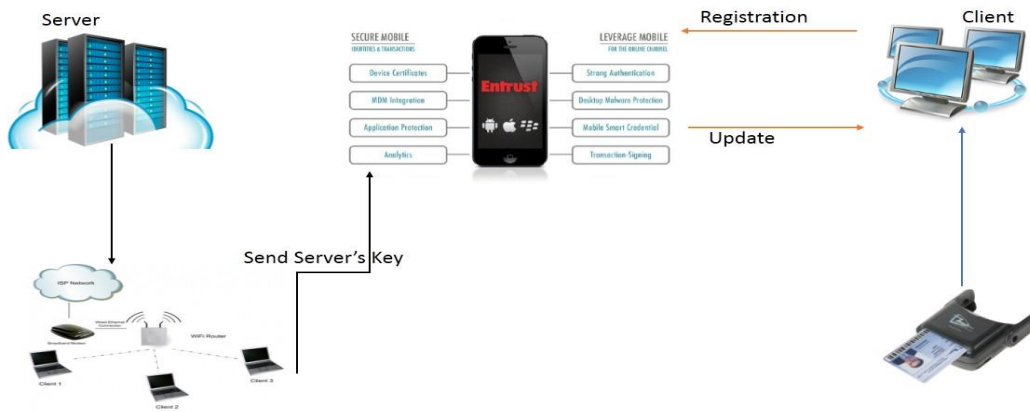
Figure 1: Architecture Diagram
