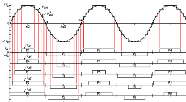
Fig2: Low loss low switching frequency multilevel inverter waveforms.
