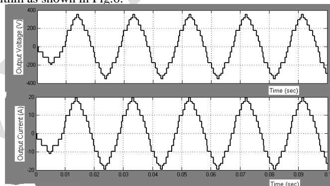
Fig 5: Output of 15 Levels multilevel Inverter
