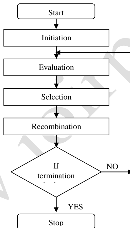
Fig 3: Flowchart of Genetic Algorithm
