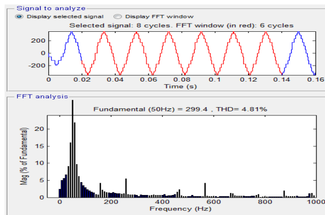
Fig 6: FFT Analysis of 15 Levels Multilevel Inverter
