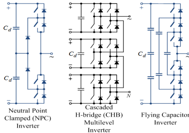
Fig 1: Multilevel Inverter Topologies
