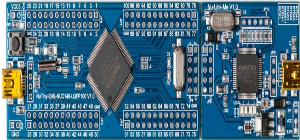
Fig 2.1. Nuvoton controller NUC140VE3CCN
