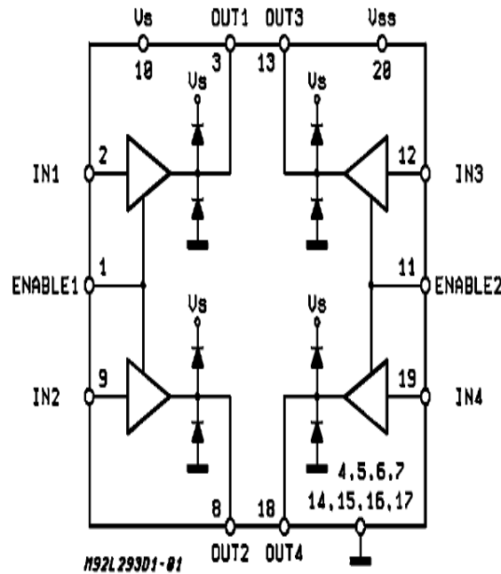
Fig 2.4. Circuit Diagram Of L293D and L293DD Chip
