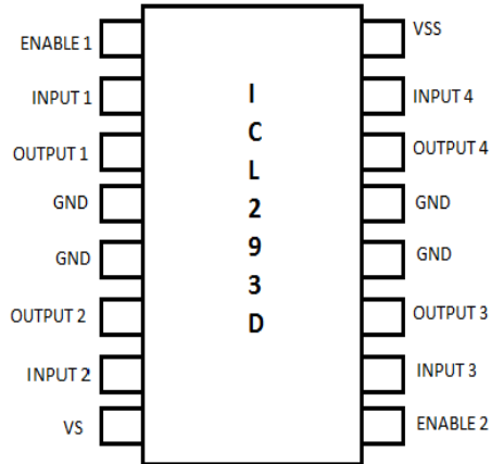
Fig 2.2 Pin Diagram Of L293D With 16 Pins
