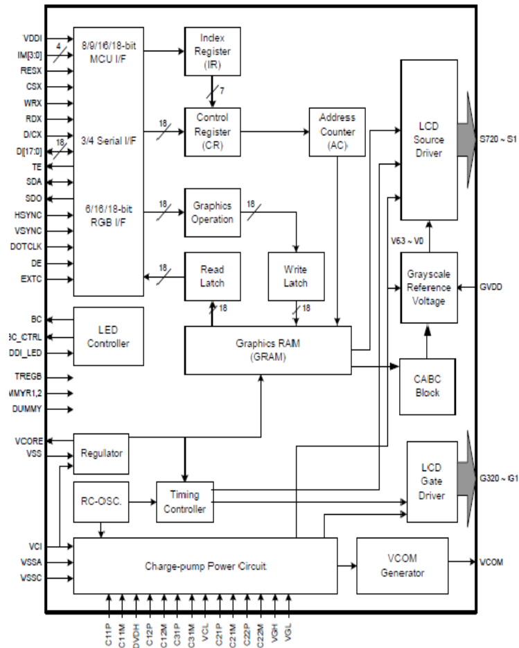
Fig2.7. Block Diagram of Touch Screen Driver
