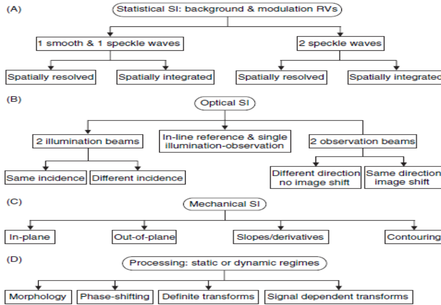
Fig.2 Different types of Speckle Interferometry
