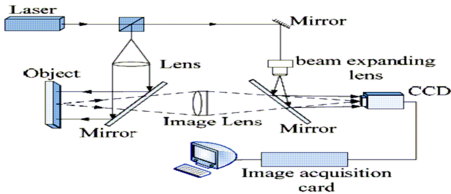
Fig.1 Laser speckle imaging setup
